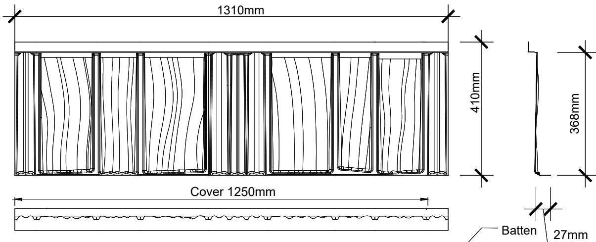
Tile Dimensions
