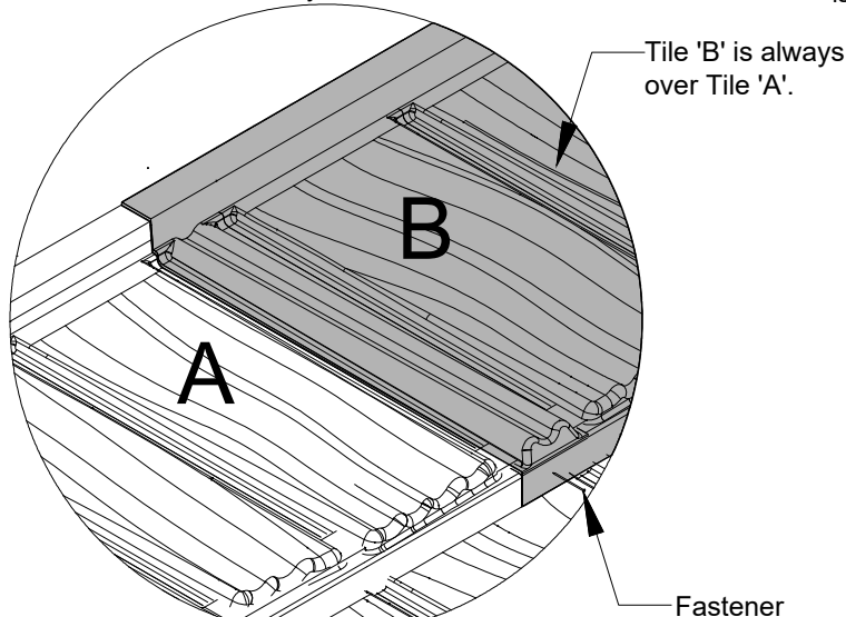
Overlap Detail
