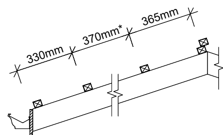
Batten Layout
